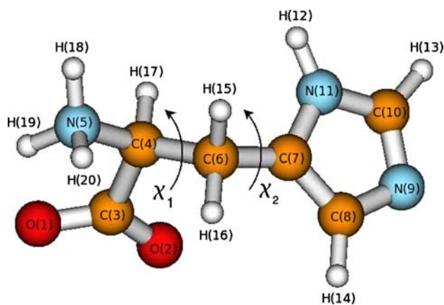
Fig. 1 Numbering scheme and definition of dihedral angles of the L-histidine zwitterion
