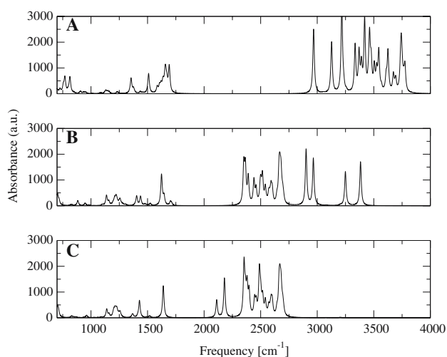
Fig. 10 Vibrational absorption spectra of the L-histidine zwitterion gmm conformer calculated at the 6-31G(d,p) level in the LH13C model with no deuterium substitution (A), deuterium substitution in solvent molecules only (B) and deuterium substitution in both solvent molecules and L-histidine (C)
